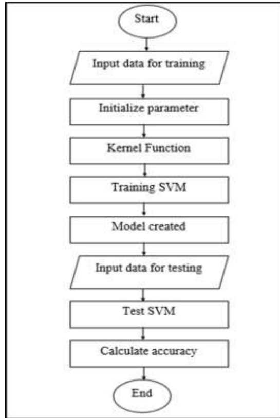
Figure 1. SVM Implementation steps
